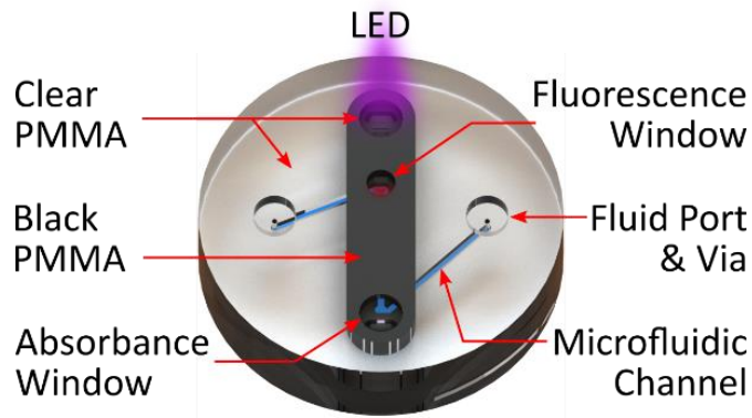
Inlaid Microfluidic Optics™ for multi-channel Fluorescence and Absorbance
